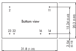
Standard pinning
