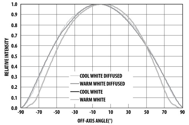
Figure 4. Radiation Pattern
