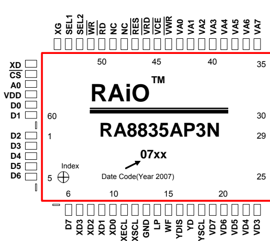
Figure 4-1: RA8835AP3N(QFP-60 Pin)
