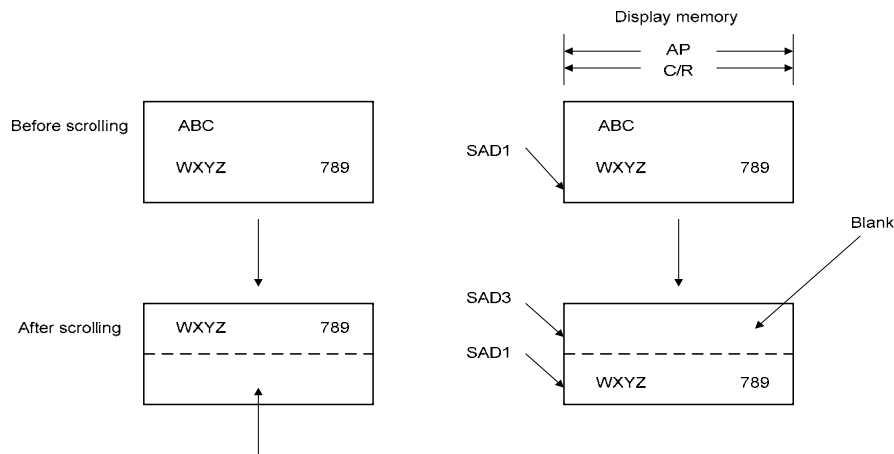
Figure 7-23: On-page Scrolling
