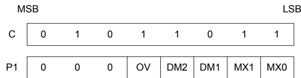
Figure 6-17: OVLAY Parameters
