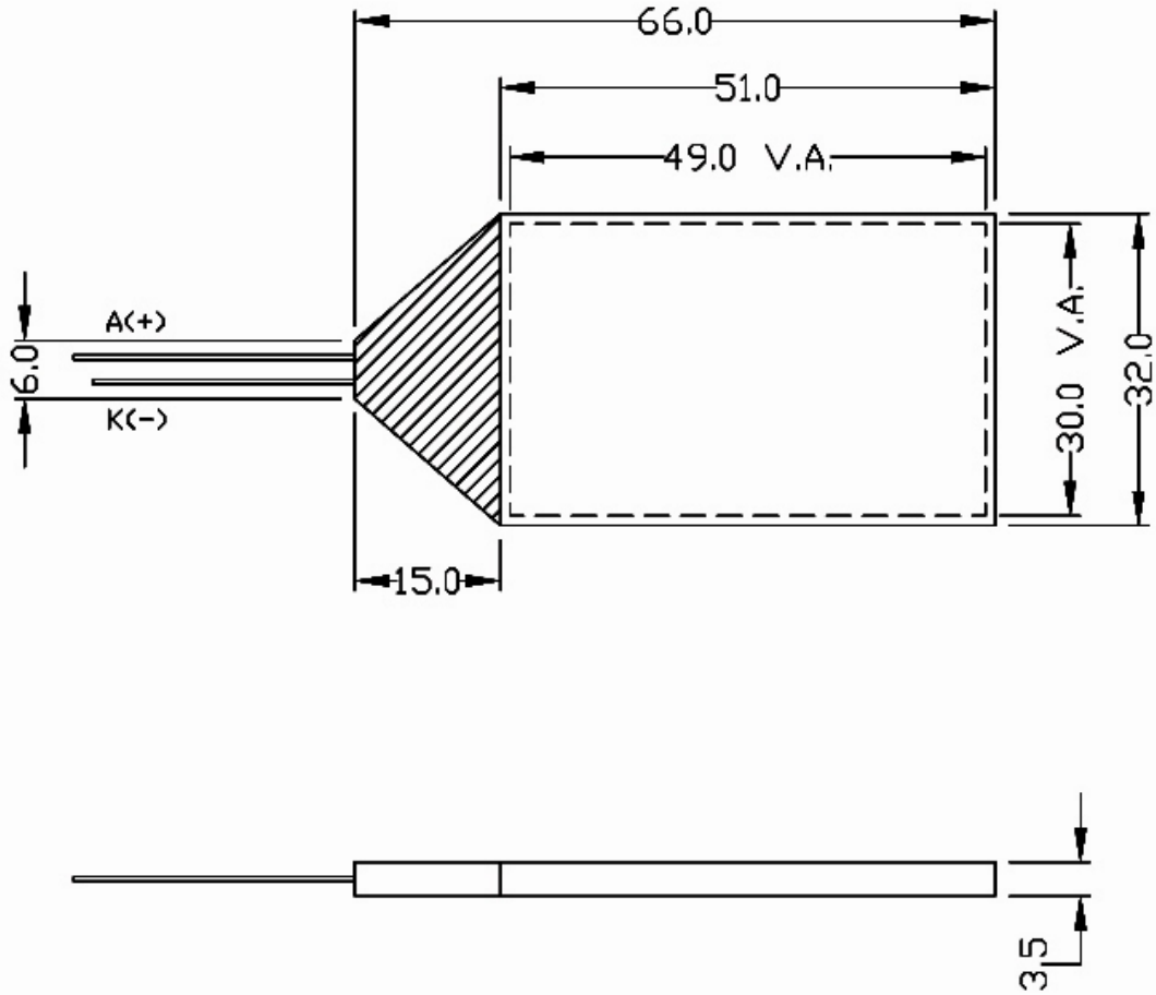
Outline Drawing Unit : mm
