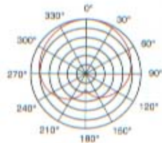
Uni-directional 单指向 (at 1kHz)
