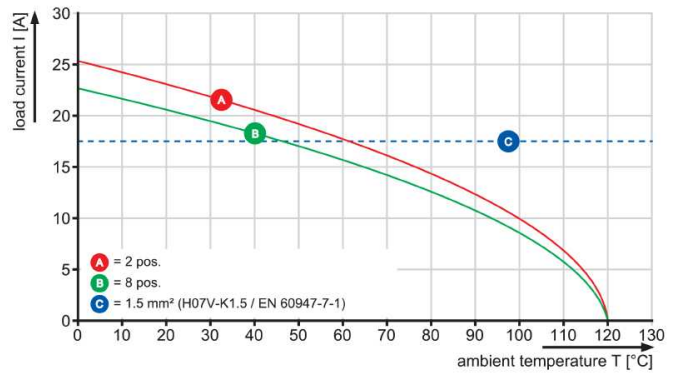
LSF-SMT 5.08/./90 3.5
