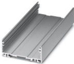
Panel mounting base, Lower part, Color: aluminum, Width: 45 mm, Constructional height: 28.1 mm
