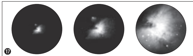
Orion-nevel (M 42)
